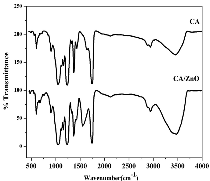
Fig. 4. FTIR spectra of (a) pure CA fibrous membrane and (b) ZnO embedded CA fibrous membrane.
