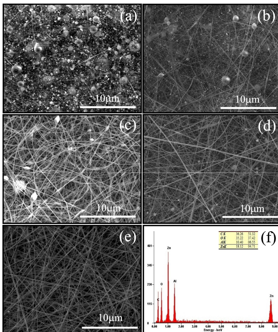
Fig. 1. SEM image of the ZnO embedded CA membrane with varied polymer concentrations: (a) 6 wt%, (b) 8 wt%, (c) 10 wt%, (d) 12 wt%, (e) 14 wt%, and (f) energy dispersive X-ray spectra analysis (EDAX).
