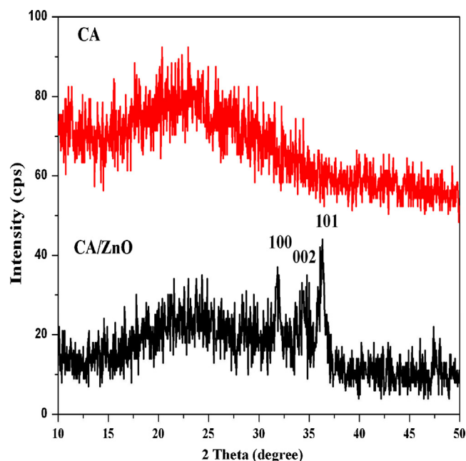
Fig. 3. XRD pattern of (a) cellulose acetate fibrous membrane and (b) ZnO embedded cellulose acetate fibrous membrane.
