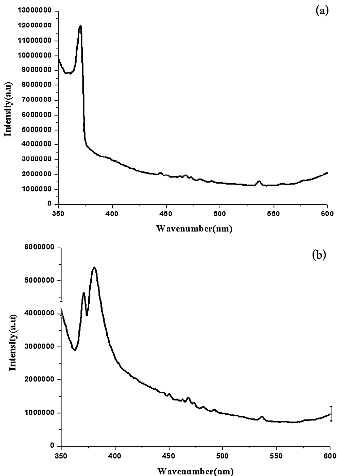
Fig. 5. PL spectra of (a) pure CA fibrous membrane and (b) ZnO embedded CA fibrous membrane.
